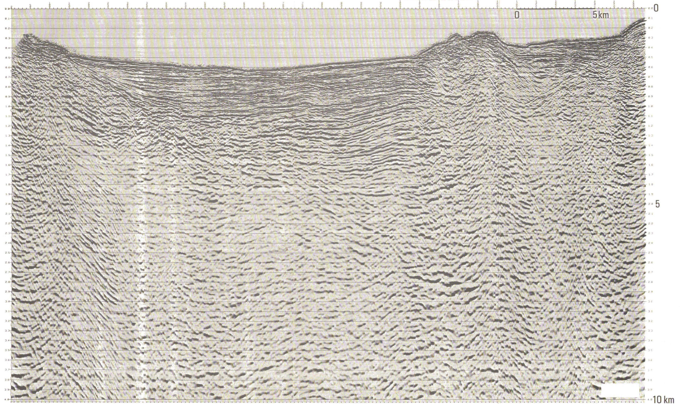
Figure 3- A Migrated depth sections, Lines A-I. Location is indicated in Figure 1. Vertical exaggeration 2.5x.
